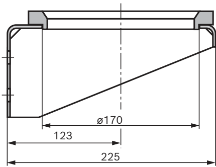
Rubber support ring (material number: 1530221042)
