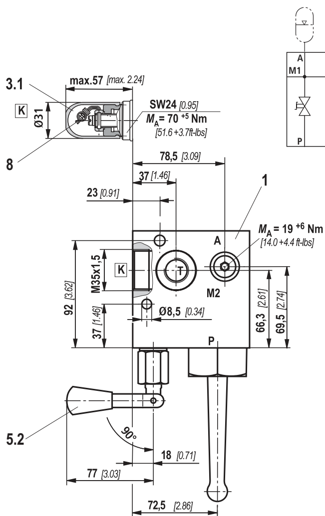
View "Z"
