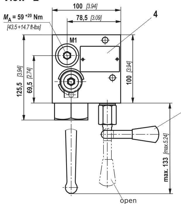
View "Z"
