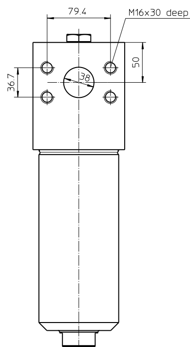
execution SAE-connection 1 1/2"
