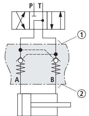
Circuit example, schematic
