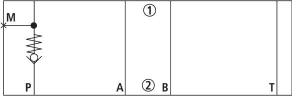
Type Z1S 6 P .-4X/... SO118 (check valve in channel P, measuring port P Out G1/4)
