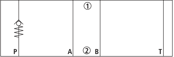
Type Z1S 6 P .-4X/... SO104 (check valve in channel P, direction of flow P1 → P2)
