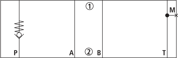
Type Z1S 6 P .-4X/... SO2 (check valve in channel P, measuring port T G1/4)
