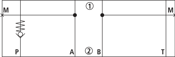
Type Z1S 6 P .-4X/... SO90 (check valve in channel P, measuring port A and B G1/4)
