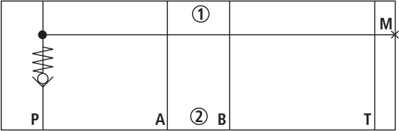
Type Z1S 6 P .-4X/... SO68 (check valve in channel P, measuring port P Out G1/4)
