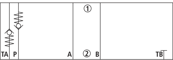
Type Z1S 10 P .-1 TA -2 TB9 -4X/... (check valve in channel TA and P, TB locked)
