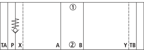
Type Z1S 10 P .-1-4X/F/ XY ... (check valve in channel P, additionally channel X and Y)
