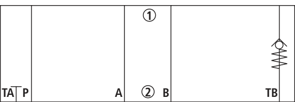
Type Z1S 10 TA .-2- TB9 -4X/... (check valve in channel TA, TB locked)
