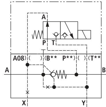
With directional seat valve type M-3SEW 6 U...
