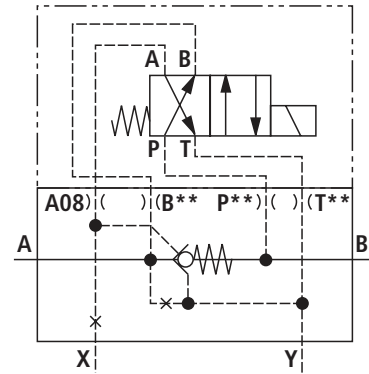
With directional spool valve type 4WE 6 Y...
