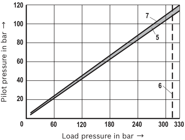
Pilot pressure/load pressure characteristic curves without pre-opening
