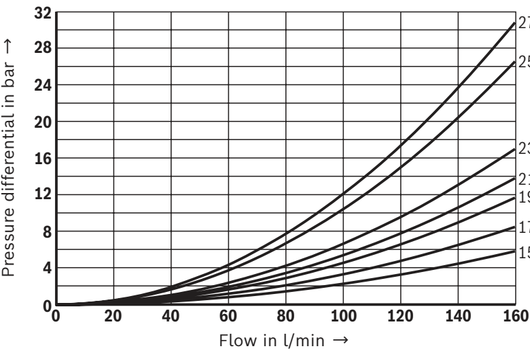
\Delta p - q_v characteristic curves
