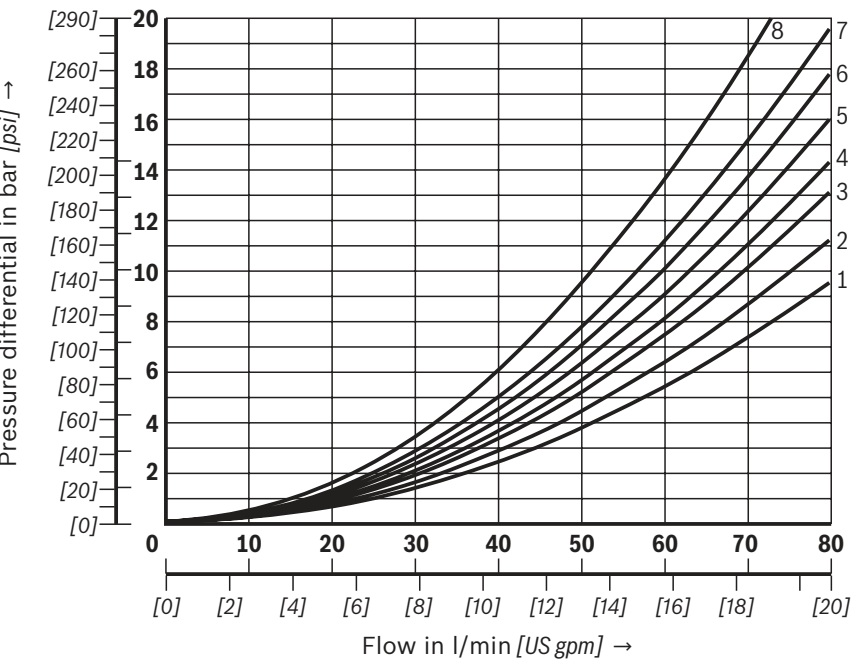
Δp-qv characteristic curves
