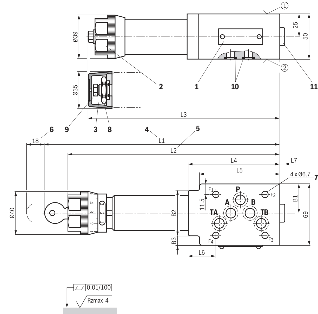
Required surface quality of the valve contact surface
