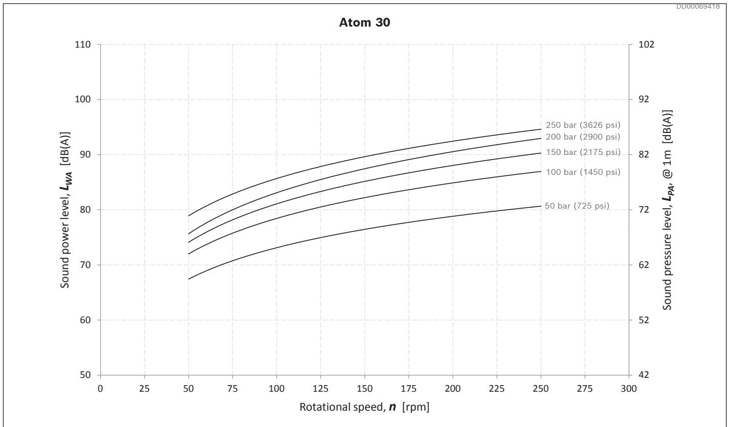
Fig. 45: Sound level Atom 30
