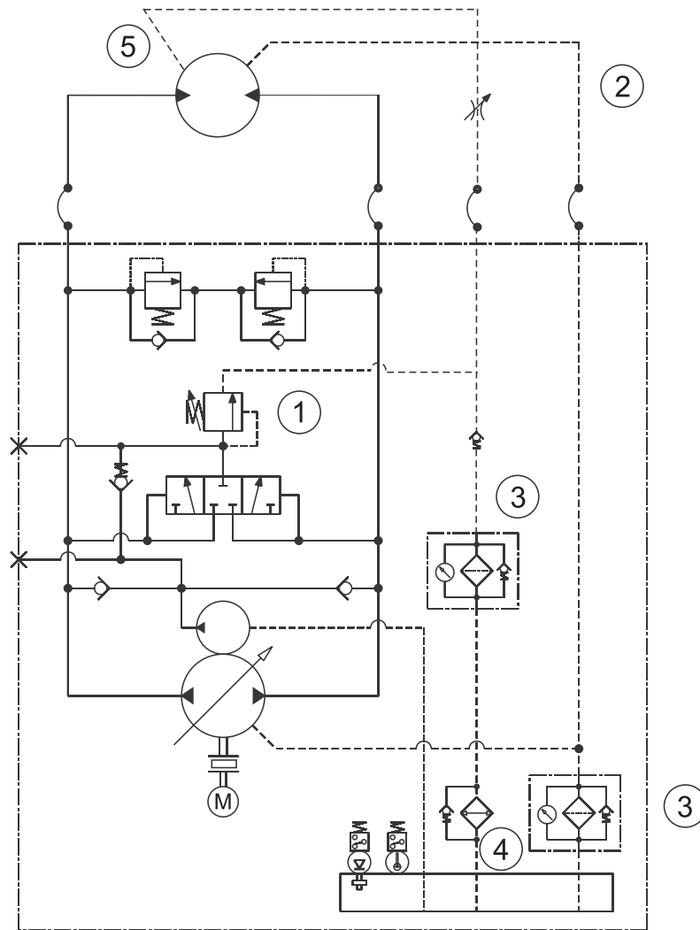
Fig. 69: Simplified closed circuit design example
