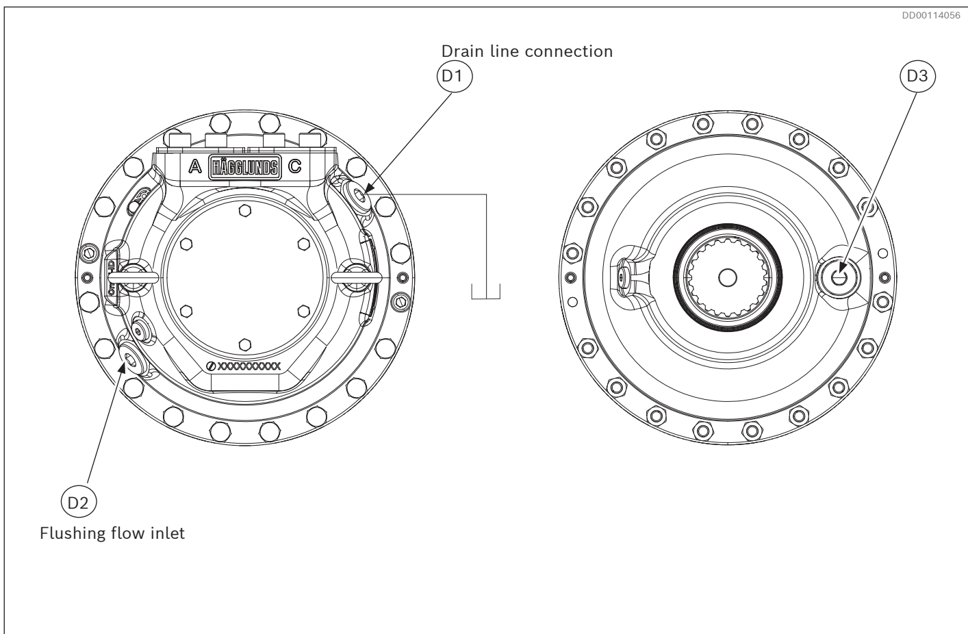
Fig. 23: Horizontal mounting
