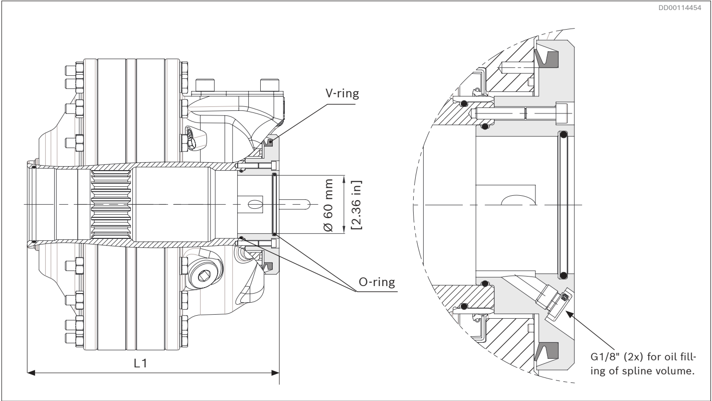
Fig. 47: Example: Hägglunds Atom 20 with through hole kit.
