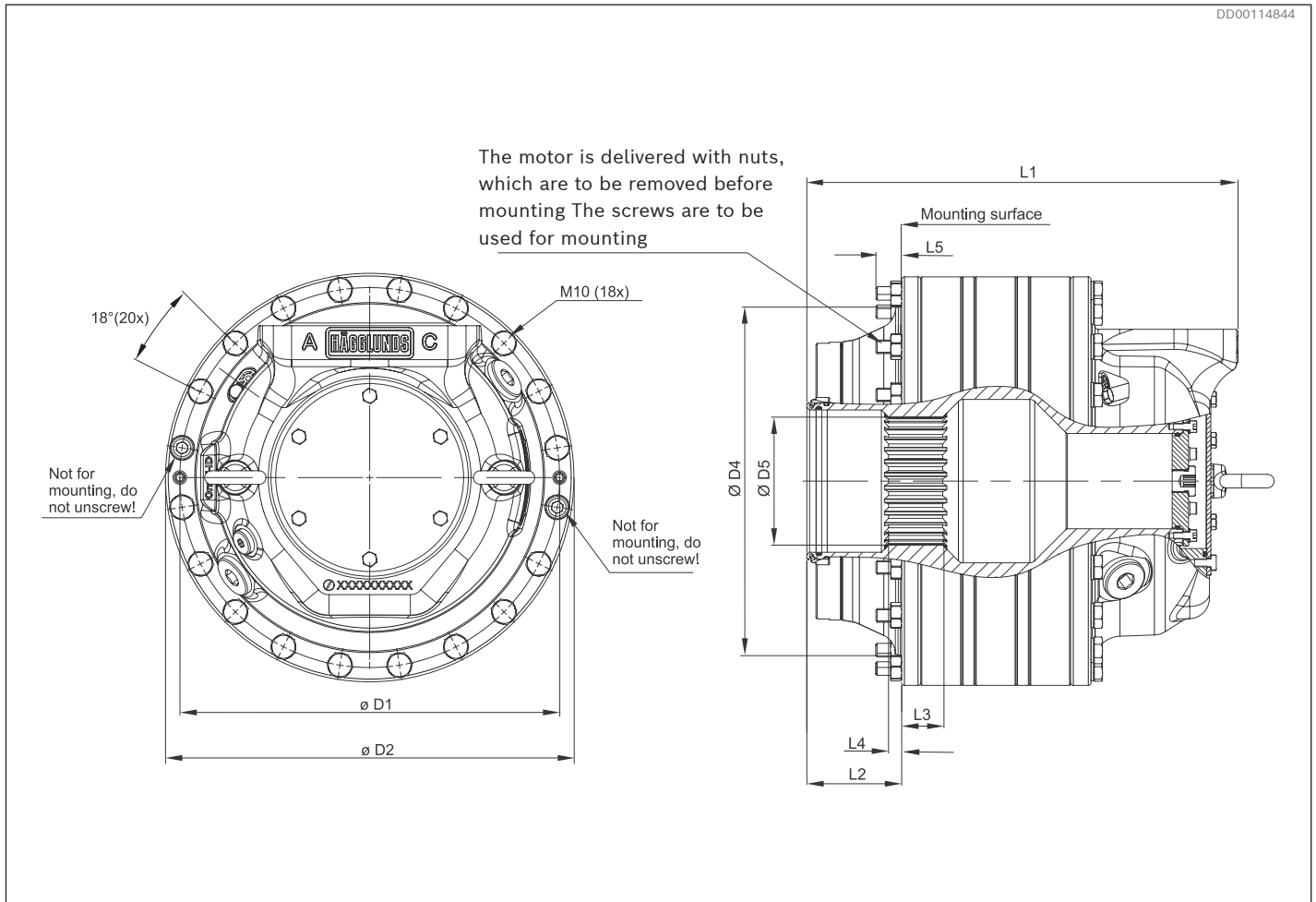
Fig. 58: Atom 30 28 F and Atom 30 30 F (front flange)
