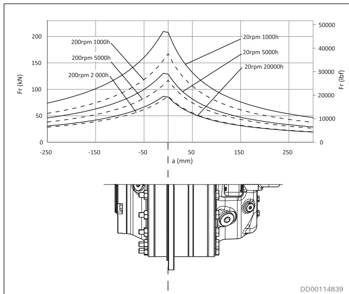
Fig. 54: Permissible external dynamic load for Atom 30 C special index 06
