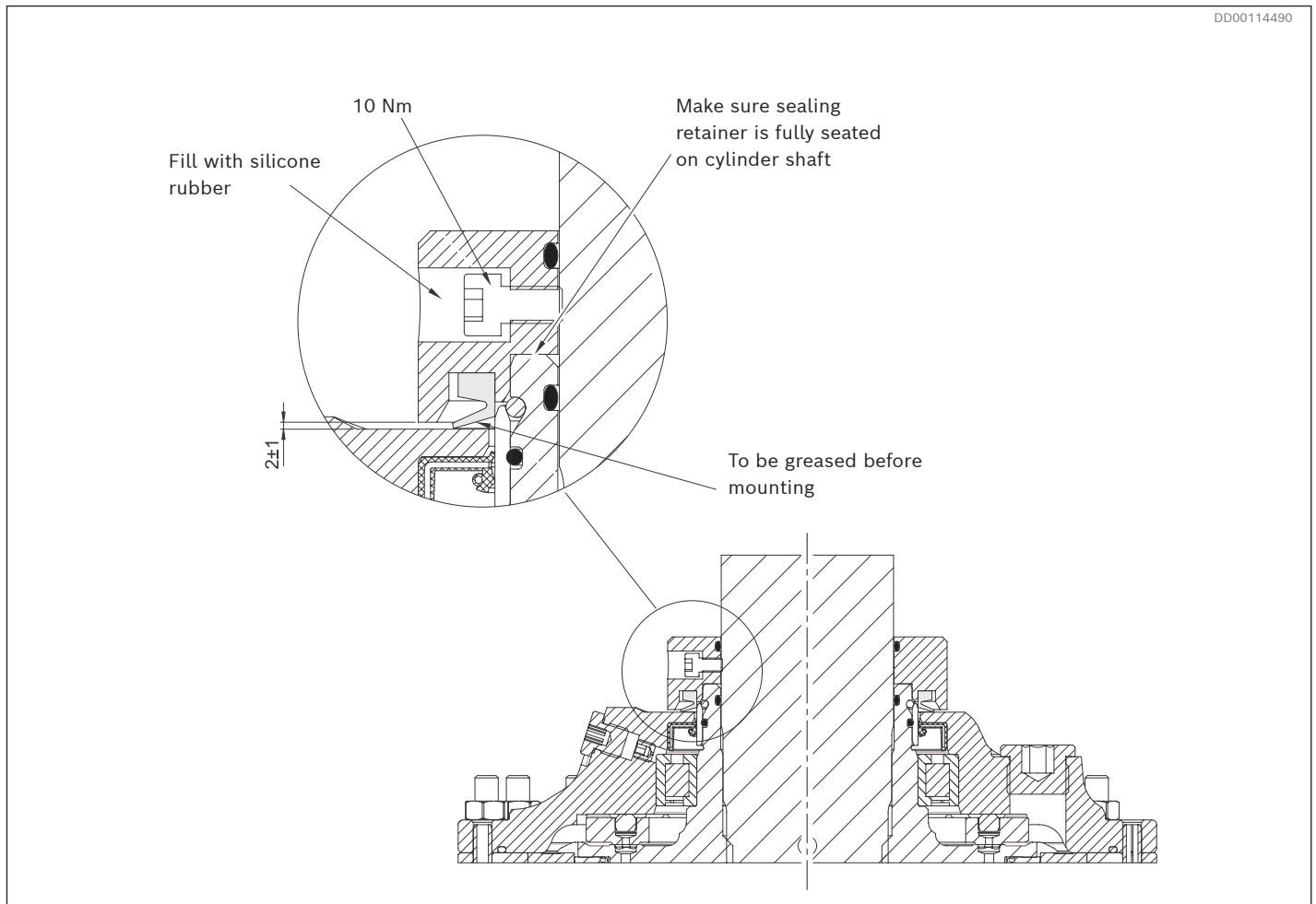
Fig. 67: Kit for harsh environment
