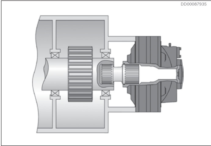
Fig. 64: Example: Flange mounted motor with spline to avoid high radial load from driven shaft.
