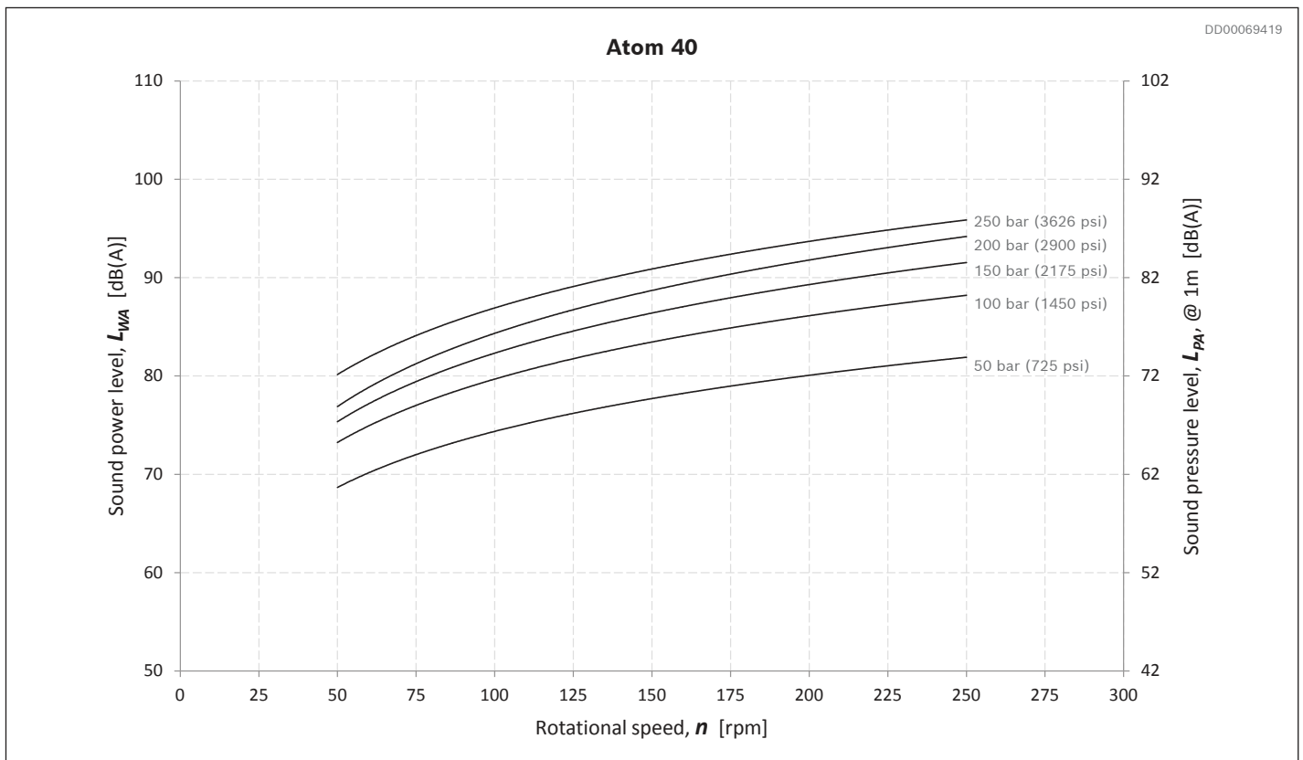
Fig. 46: Sound level Atom 40
