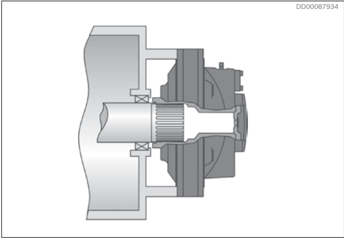
Fig. 63: Example: Flange mounted motor with spline and low radial load from driven shaft.
