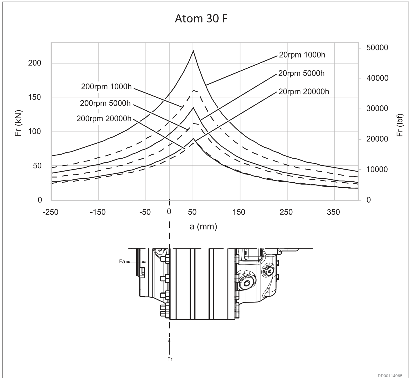
Fig. 34: Permissible external dynamic load Hägglands Atom 30 28 F and Atom 30 30 F (front flange)
