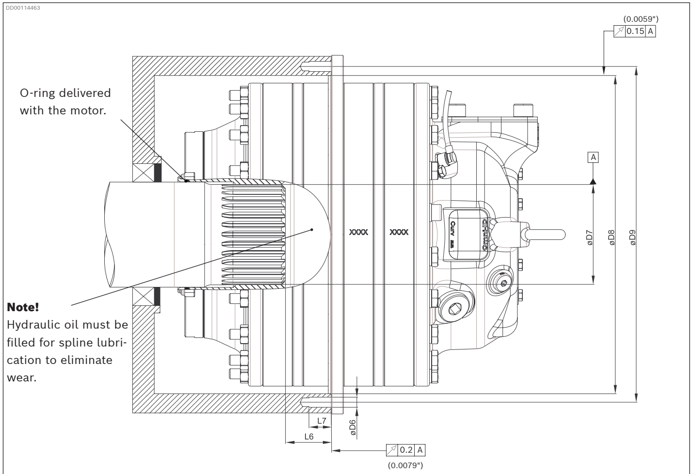
Fig. 62: Shaft installation tolerances Atom 30 C (center flange), Atom 40
