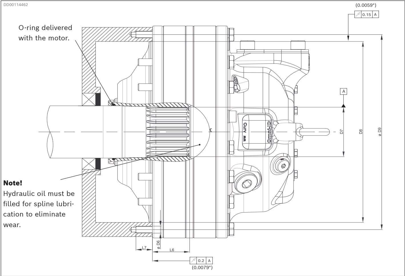
Fig. 61: Shaft installation tolerances Atom 10, Atom 20, and Atom 30 F (front flange)
