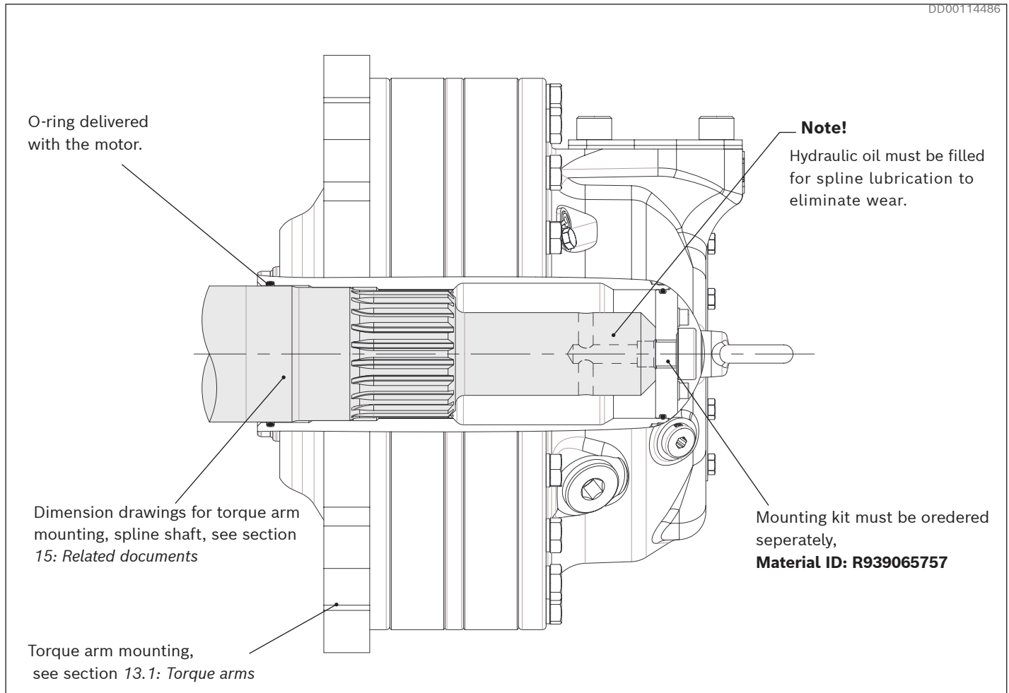
Fig. 65: Example: Torque arm mounting of Atom 20
