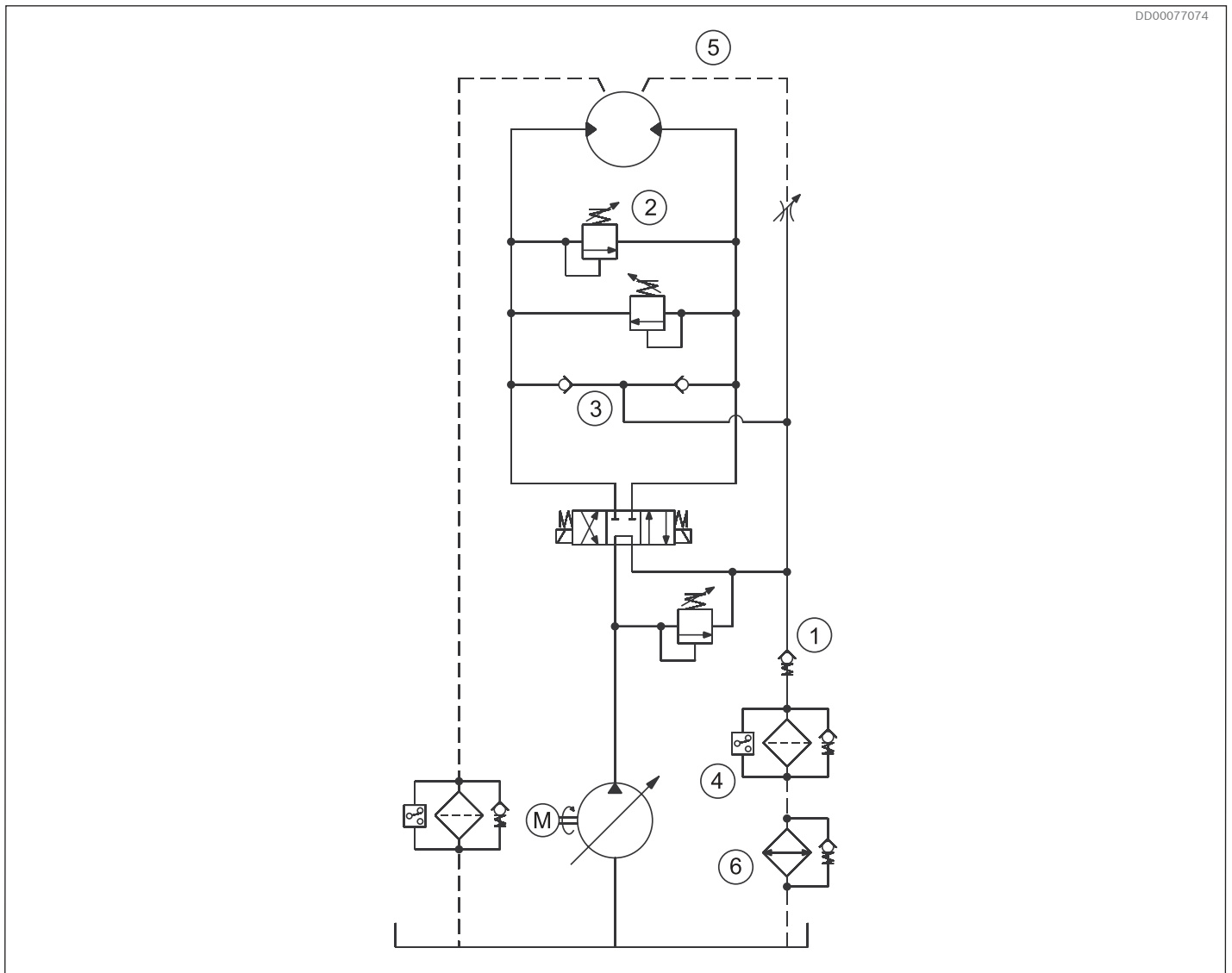
Fig. 68: Simplified open circuit design example
