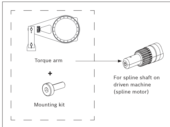
Fig. 66: Single ended torque arm mounting for spline shaft
