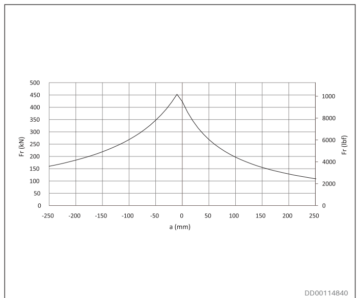
Fig. 55: Permissible external static load for Atom 30 C special index 06
