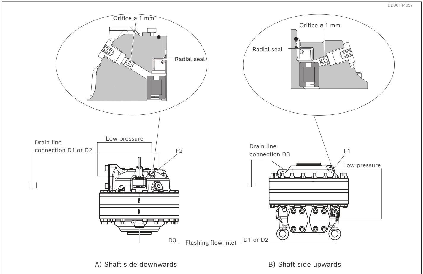
Fig. 24: Vertical mounting
