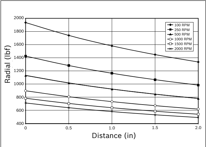
Load from mounting plate at 3000 hrs L_{10} bearing life
