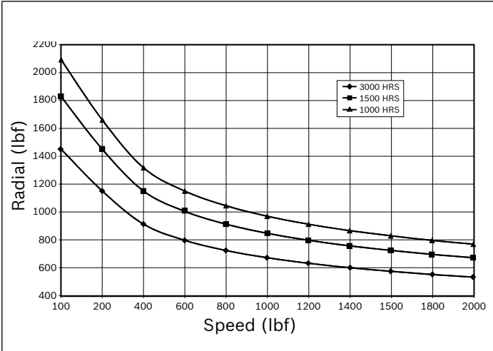
Bearing load at center of output shaft
