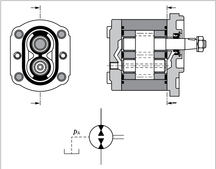
▼ Reversible gear motor
