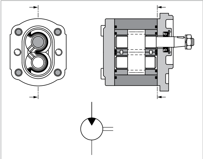
▼ Gear motor for one direction of rotation
