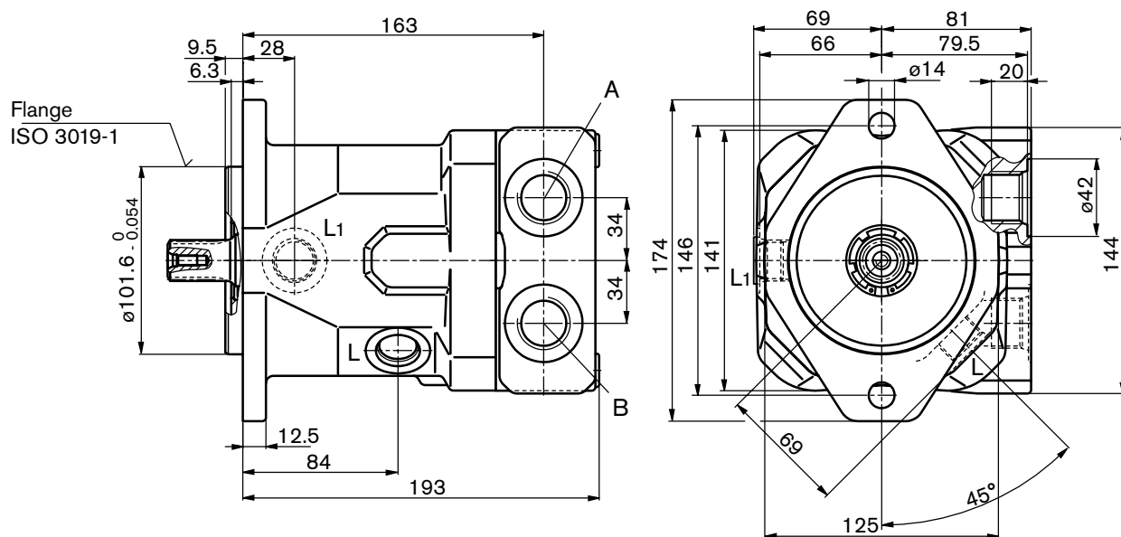
Port plate 16
