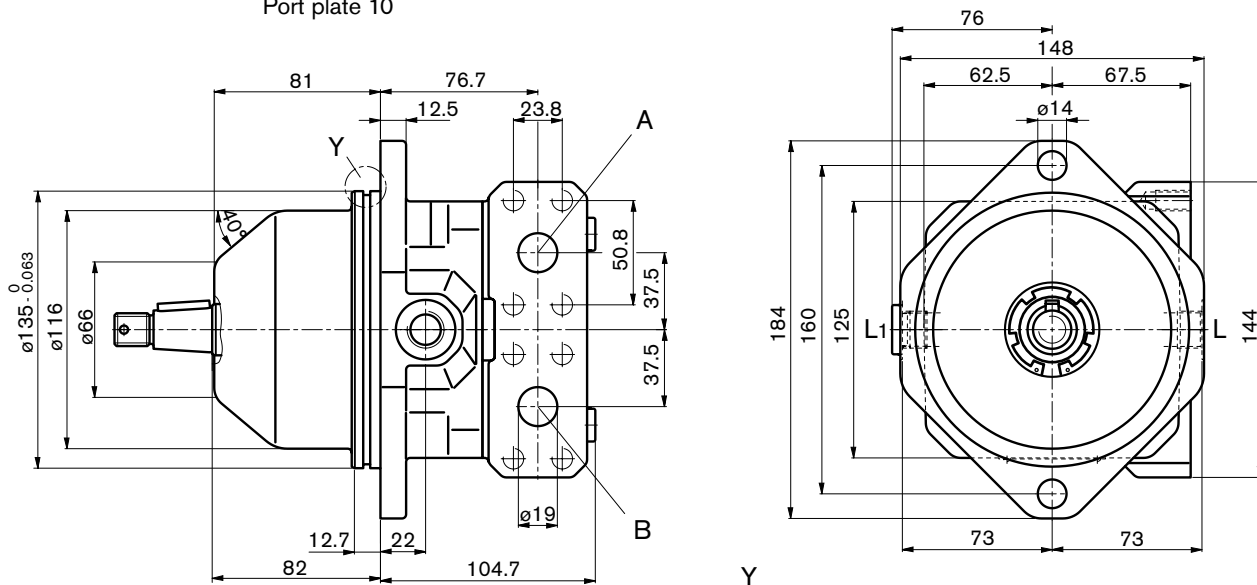
Port plate 10
