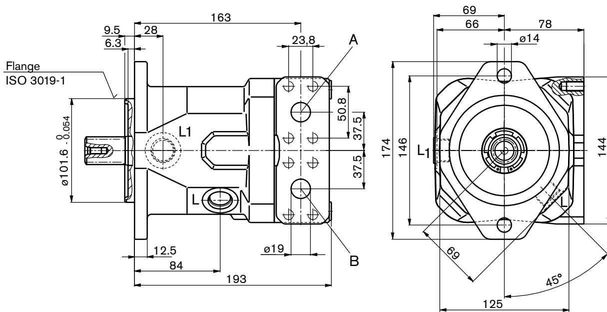
Port plate 10
