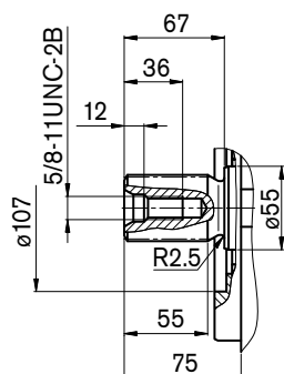
S Splined shaft SAE J744 1 3/4 in 13T 8/16DP 3)
