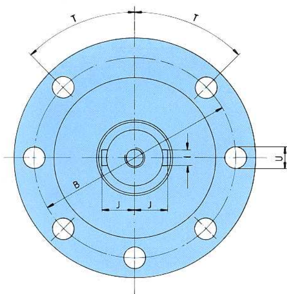
View A
