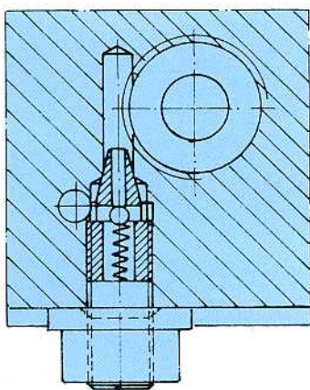
14 Adjustment of cushioning
