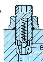
Throttle non-return valve
